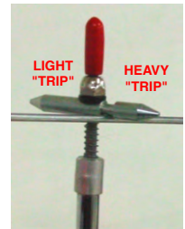
INSET "A" TRIP-SHAFT
